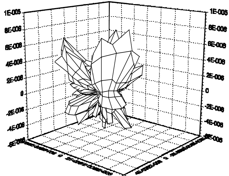
DEC 1998 NSWCD ANECHOIC CHAMBER LAPTOP COMPUTER RADIATED EMISSIONS MSMTS 601 MHz, HOR POL
